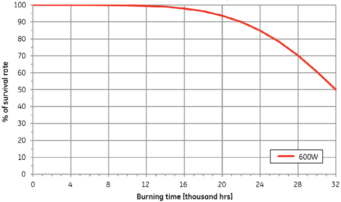
Survival rate of XO 600W lamp
