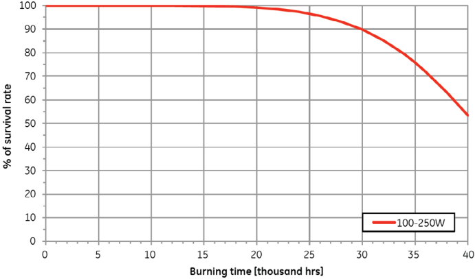
Survival rate of XO 100W lamp
